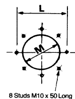
Boiler Frontplate drilling
